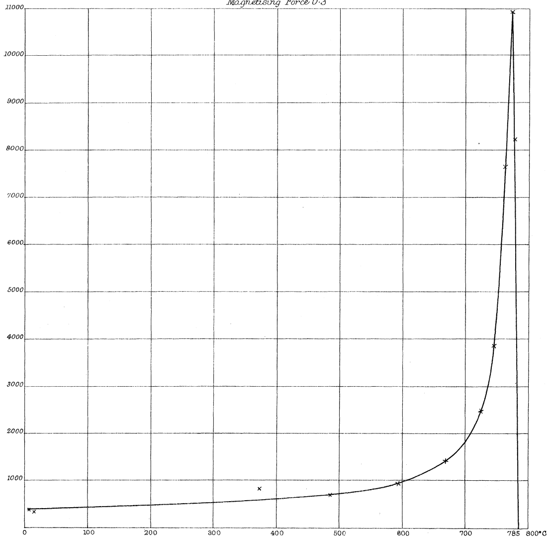
Wrought Iron. Curve XII. Magnetising Force 0.3
