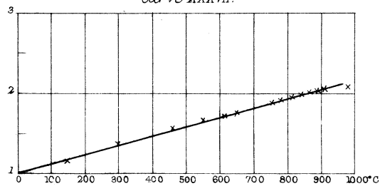
Manganese Steel Wire. Curve XXXVII.
