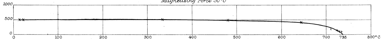
Curve XXII. Magnetising Force 30.0.
